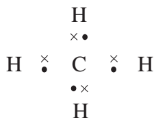
Dot and cross diagram of methane
