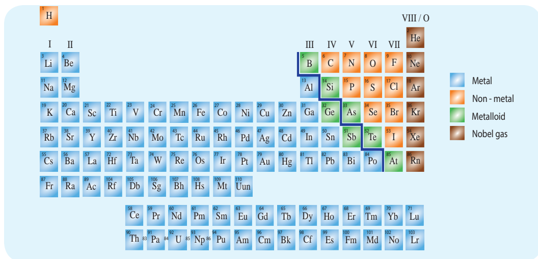
Fig. 3.11 - The modern Periodic Table
