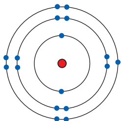
Fig. 10.3 A chlorine atom
