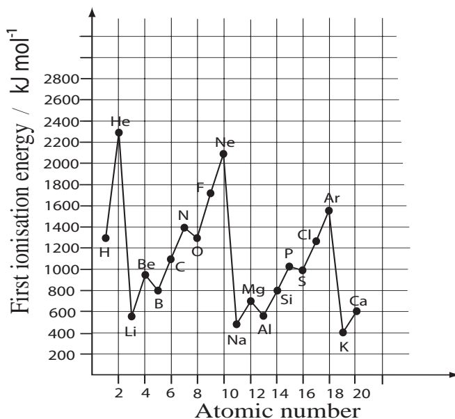
Fig. 3.8 - The graph of ionisation energy variation against atomic number for first 20 elements
