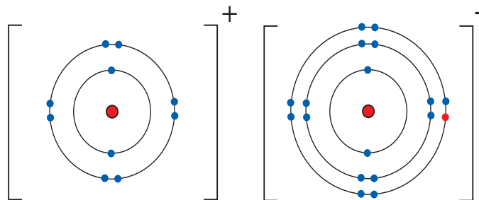
Fig.10.5 Electrostatic attraction between Na + and Cl - ions
