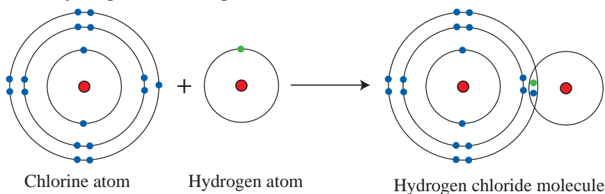
Fig. 10.13 Formation of a hydrogen chloride molecule
