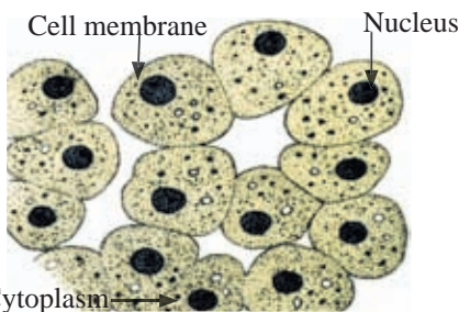
Figure 6.4 (a) - Animal cells
