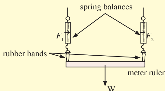
Figure 12.10 - Equilibrium of a meter ruler under three coplanar parallel forces
