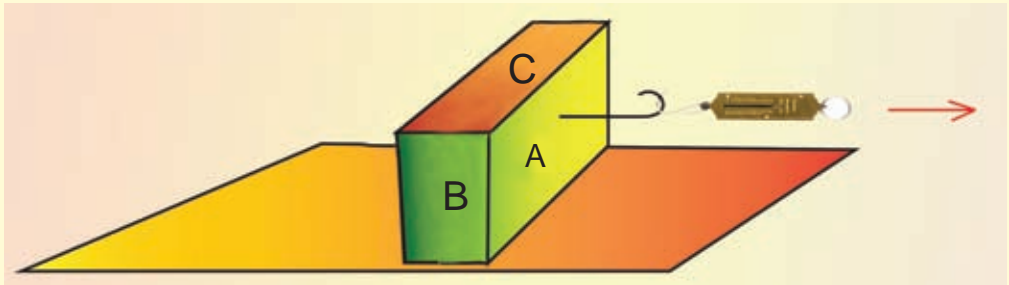
Figure 5.4 – Investigation of the influence of surface area on friction
