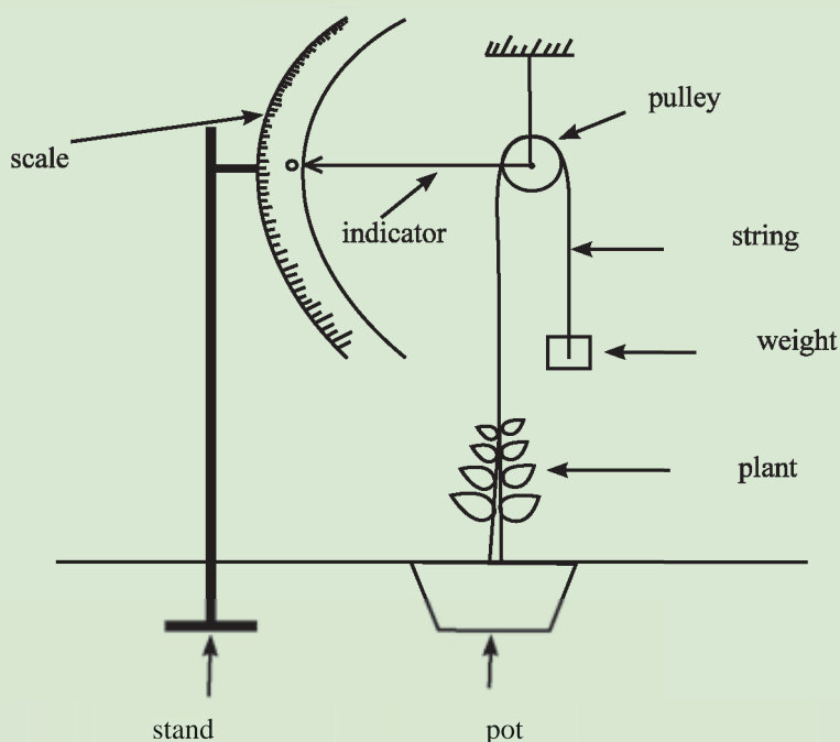
Figure 8.12- A model of an auxanometer
