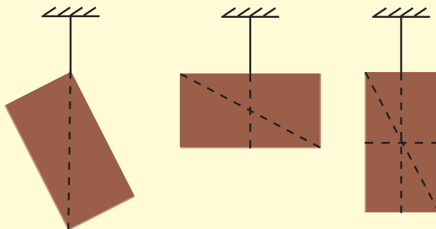
Figure 12.13 - Finding the centre of gravity of the laminar
